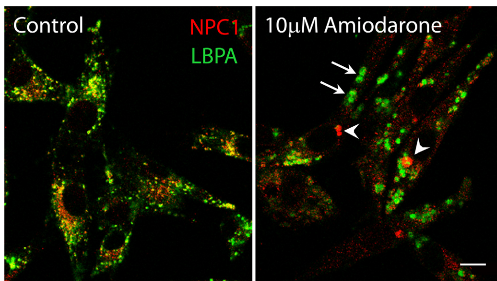
Fig. 10. Amiodarone induces aggregates of NPC1 protein spatially separated from aggregates of LBPA. BHK cells incubated for 16 h with 0 or 10 \mu M amiodarone were stained with antibodies to NPC1 and LBPA and then were analyzed with confocal microscopy. Arrowheads indicate aggregates of NPC1 (red). Arrows indicate aggregates of LBPA (green). Yellow indicates co-localization.
