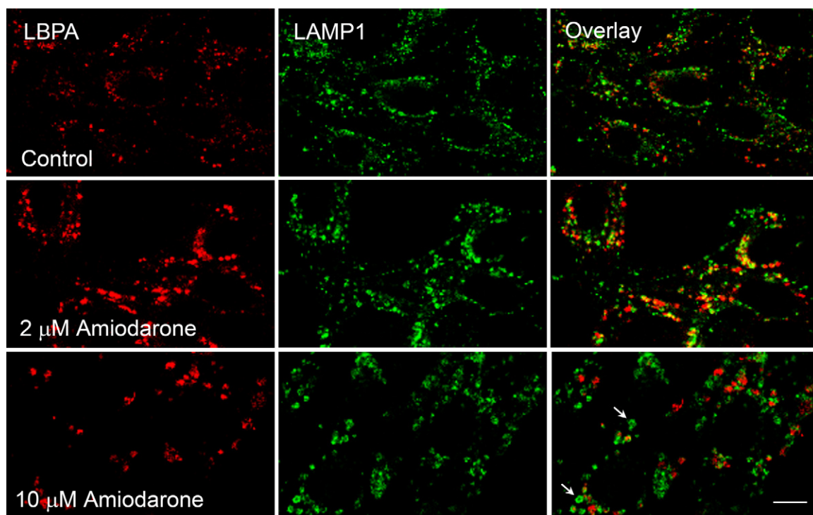
Fig. 8. Effect of amiodarone on the distribution of LAMP1 and LBPA. BHK cells, incubated for 16 h with 0–10 \mu M amiodarone, were stained with antibodies to LAMP1 and LBPA and then were analyzed with confocal microscopy. Arrows: ring-like structures containing LAMP1. Bar 10 \mu m.
