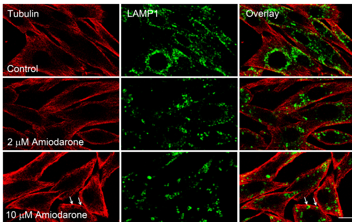
Fig. 9. Effect of amiodarone on the distribution of LAMP1 and tubulin. BHK cells, incubated for 16 h with 0–10 \mu M amiodarone, were stained with antibodies to LAMP1 and tubulin and then were analyzed with confocal microscopy. Arrows: aggregates of LAMP1 surrounded by a rim of tubulin. Bar 10 \mu m.
