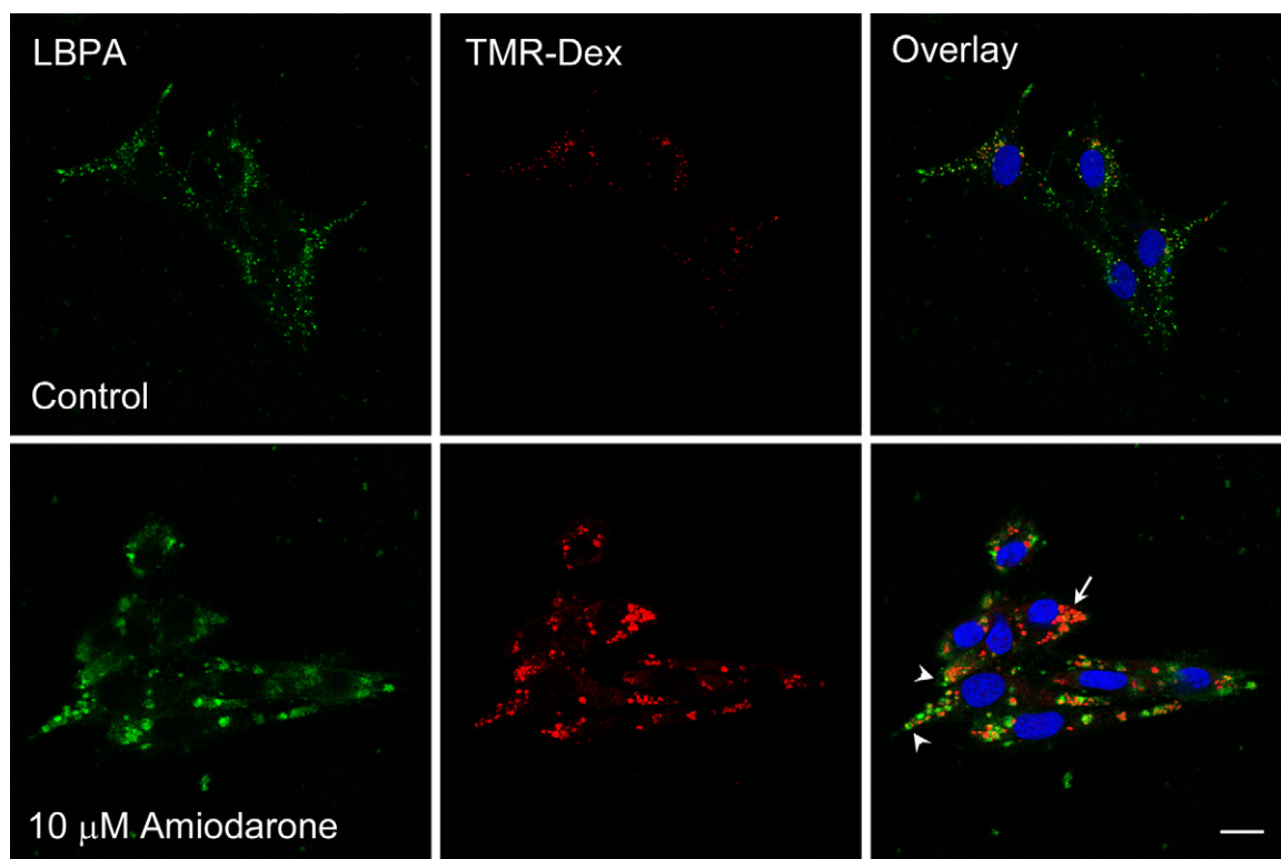
Fig. 7. Amiodarone alters fluid phase endocytosis. BHK cells were loaded for 12 h with tetramethylrhodamine dextran (TMR-Dex) and then were chased for 5 h either with or without 10 \mu M amiodarone. The distribution of TMR-Dex (red) and LBPA (green) was then analyzed by confocal microscopy. Nuclei stained blue. Arrows indicate dilated vacuoles containing TMR-Dex. Arrowheads indicate TMR-Dex and LBPA co-localization (yellow). Bar 10 \mu m.
