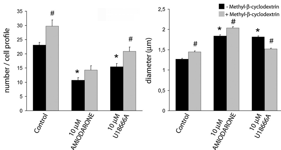
Fig. 6. Cholesterol removal alleviates the change in LBPA distribution induced by U18666A, but not that induced by amiodarone. BHK cells were incubated for 24 h with control medium or 1 mM methyl- \beta -cyclodextrin and then for further 16 h with control medium, 10 \mu M amiodarone or 10 \mu M U18666A. At the end the distribution of LBPA was analyzed by confocal microscopy and number and diameter of LBPA-positive structures were measured. M \pm SE . *Different from control, # different from same treatment without methyl- \beta -cyclodextrin ( p < 0.05 , ANOVA).
