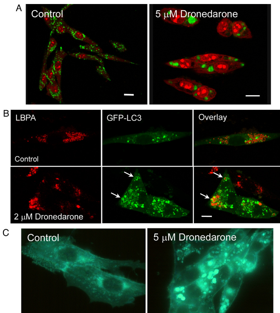
Fig. 11. Dronedarone alters the distribution of LBPA and unesterified cholesterol and stimulates autophagy. (A) Confocal images of BHK cells incubated for 16 h with 5 \mu M dronedarone, stained for LBPA (green) and then counterstained with propidium iodide (red). (B) BHK cells, transiently transfected with pEGFP-LC3 plasmid, were incubated for 16 h with control medium or with 2 \mu M dronedarone. The distribution of LBPA (red) and LC3 (green) was then analyzed by confocal microscopy. Arrow: LC3 positive membranes surrounding LBPA aggregates. (C) Epifluorescence image of BHK cells incubated for 16 h with 0 (control) or 5 \mu M dronedarone and then incubated with filipin to stain unesterified cholesterol.
