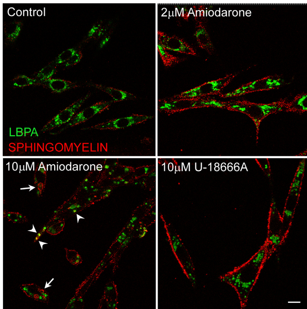
Fig. 4. Amiodarone changes the distribution of sphingomyelin. BHK cells, exposed for 16 h to control medium, 2 or 10 \mu M amiodarone or 10 \mu M U18666A, were fixed, incubated first with the sphingomyelin-binding protein lysenin and then with antibodies to lysenin and LBPA. After incubation with secondary antibody cells were analyzed by confocal microscopy. Red, sphingomyelin; green, LBPA. Arrows indicate sphingomyelin in intracellular structures. Arrowheads indicate co-localization of sphingomyelin and LBPA (yellow). Bar 10 \mu m.
